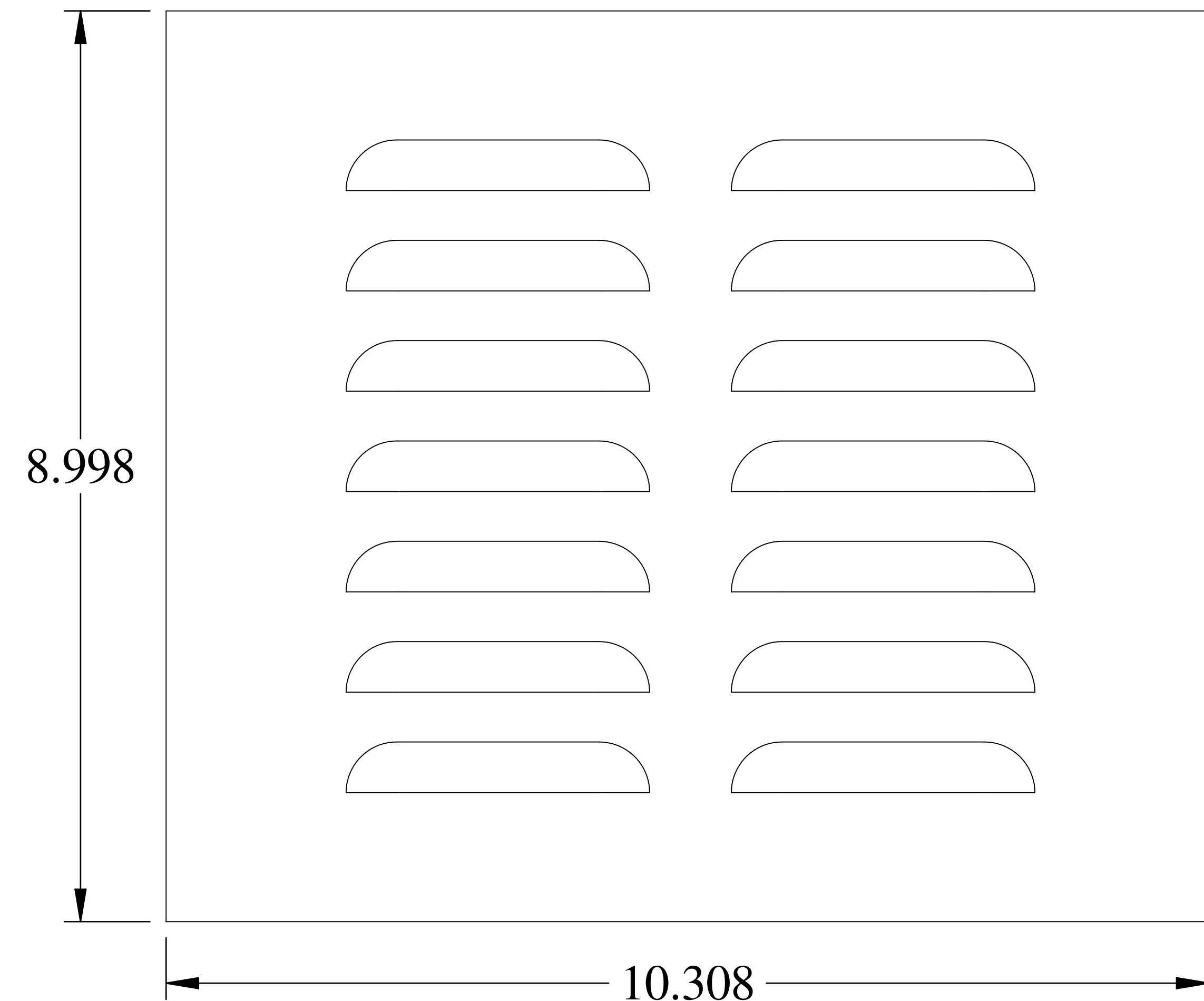
FRONT VIEW
